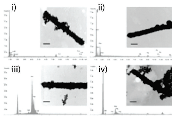
Figure 4. (A) Electroless deposition. Transmission electron micrographs of metalized TMV particles produced by electroless deposition. (i) TMV after Pd(II) activation, followed by electroless deposition of Ni. TMV is filled with a nickel wire with a ca. 3 nm diameter. Reproduced with permission from ref 80. Copyright 2003 American Chemical Society. (ii) TMV metalized with nickel on the external surface. Reproduced with permission from ref 82. Copyright 2004 Wiley. (B) Silica-templated mineralization. Transmission electron micrographs and accompanying energy dispersive X-ray spectra of (i) Au on thick-shell silica-coated TMV template, (ii) Ag on thick-shell silica-coated TMV template, (iii) Pt on thick-shell silica-coated TMV template, and (iv) Pd on thick-shell silica-coated TMV template. Al, Fe, and Cu peaks in the energy dispersive spectroscopy spectra are due to background effects. Scale bar = 100 nm. Reproduced with permission from 84. Copyright 2009 Elsevier. (C) M13 heterostructures. (i–v) Transmission electron micrographs of various nanoarchitectures templated by M13. Gold nanoparticles (~5 nm) bind to genetically engineered pVIII proteins along the virus axis and form 1D arrays, while a second peptide motif on pIII protein simultaneously binds to streptavidin-coated nanoparticles. Arrows highlight the streptavidin-conjugated gold nanoparticles (~15 nm) and CdSe quantum dots bound on pIII proteins. The insets show the assembly schemes of observed structures. White represents the virus structure, yellow dots represent gold nanoparticles, the green dot represents a CdSe quantum dot, and red represents the streptavidin coating around gold or CdSe particles. (C, inset) The enlarged image of the CdSe quantum dot attached to the end of the virus. Reproduced with permission from ref 88. Copyright 2005 American Chemical Society. (D) Spatially constrained synthesis. Transmission electron micrographs of paratungstate-mineralized CCMV particles after isolation by centrifugation on a sucrose gradient. (i) An unstained sample showing discrete electron dense cores; (ii) a negatively stained sample showing the mineral core surrounded by the intact virus protein cage. Reproduced with permission from ref 12. Copyright 1998 Nature Publishing Group.
