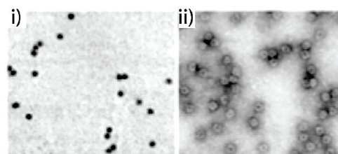
Figure 4. (A) Electroless deposition. Transmission electron micrographs of metalized TMV particles produced by electroless deposition. (i) TMV after Pd(II) activation, followed by electroless deposition of Ni. TMV is filled with a nickel wire with a ca. 3 nm diameter. Reproduced with permission from ref 80. Copyright 2003 American Chemical Society. (ii) TMV metalized with nickel on the external surface. Reproduced with permission from ref 82. Copyright 2004 Wiley. (B) Silica-templated mineralization. Transmission electron micrographs and accompanying energy dispersive X-ray spectra of (i) Au on thick-shell silica-coated TMV template, (ii) Ag on thick-shell silica-coated TMV template, (iii) Pt on thick-shell silica-coated TMV template, and (iv) Pd on thick-shell silica-coated TMV template. Al, Fe, and Cu peaks in the energy dispersive spectroscopy spectra are due to background effects. Scale bar = 100 nm. Reproduced with permission from 84. Copyright 2009 Elsevier. (C) M13 heterostructures. (i–v) Transmission electron micrographs of various nanoarchitectures templated by M13. Gold nanoparticles (~5 nm) bind to genetically engineered pVIII proteins along the virus axis and form 1D arrays, while a second peptide motif on pIII protein simultaneously binds to streptavidin-coated nanoparticles. Arrows highlight the streptavidin-conjugated gold nanoparticles (~15 nm) and CdSe quantum dots bound on pIII proteins. The insets show the assembly schemes of observed structures. White represents the virus structure, yellow dots represent gold nanoparticles, the green dot represents a CdSe quantum dot, and red represents the streptavidin coating around gold or CdSe particles. (C, inset) The enlarged image of the CdSe quantum dot attached to the end of the virus. Reproduced with permission from ref 88. Copyright 2005 American Chemical Society. (D) Spatially constrained synthesis. Transmission electron micrographs of paratungstate-mineralized CCMV particles after isolation by centrifugation on a sucrose gradient. (i) An unstained sample showing discrete electron dense cores; (ii) a negatively stained sample showing the mineral core surrounded by the intact virus protein cage. Reproduced with permission from ref 12. Copyright 1998 Nature Publishing Group.
